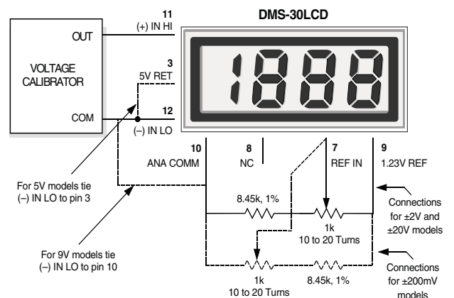
Figure 9. External Gain Adjustment
