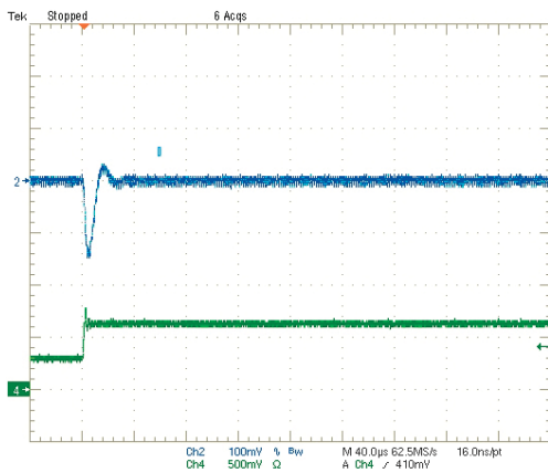
Step Load Transient Response (Vin=5V, Vout=1.0V, Cload=0, Iout=1.5A to 3A) Trace 2=Vout, 100 mV/div. Trace 4=Iout, 2.5A/div.
