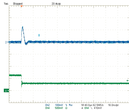
Step Load Transient Response (Vin=5V, Vout=1.0V, Cload=0, Iout=3A to 1.5A) Trace 2=Vout, 100 mV/div. Trace 4=Iout, 2.5A/div.
