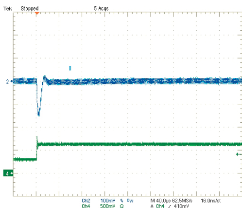
Step Load Transient Response (Vin=5V, Vout=2.5V, Cload=0, Iout=1.5A to 3A) Trace 2=Vout, 100 mV/div. Trace 4=Iout, 2.5A/div.
