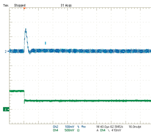
Step Load Transient Response (Vin=5V, Vout=2.5V, Cload=0, Iout=3A to 1.5A) Trace 2=Vout, 100 mV/div. Trace 4=Iout, 2.5A/div.
