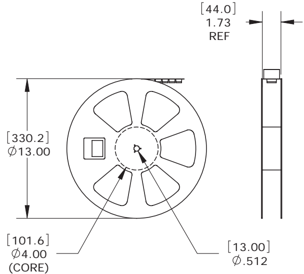
REEL INFORMATION (250 UNITS PER REEL)
