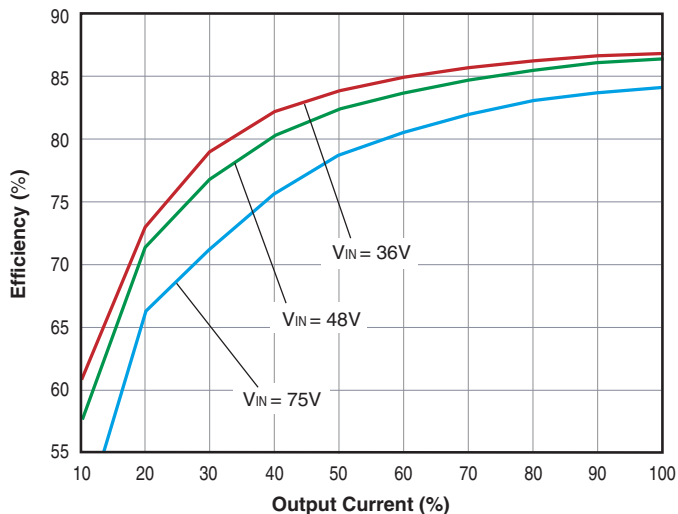
BWR-12/725-D48A Efficiency vs. Input Line And Output Load
