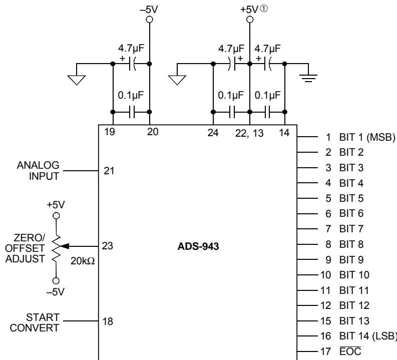
Figure 3. Connection Diagram
