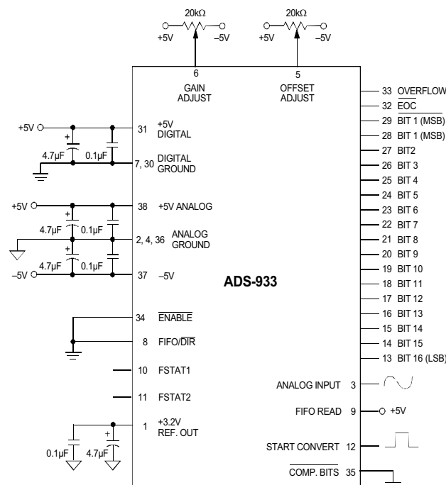
Figure 2. Bipolar Connection Diagram
