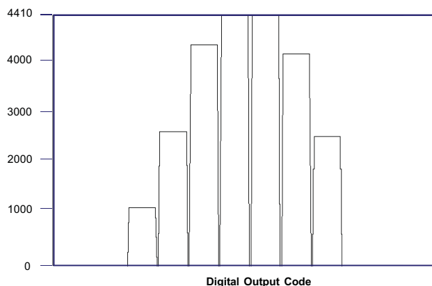
Figure 7. ADS-932 Grounded Input Histogram This histogram represents the typical peak-to-peak noise (including quantization noise) associated with the ADS-932.
