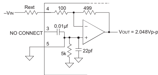
Figure 2f. Inverting Mode
