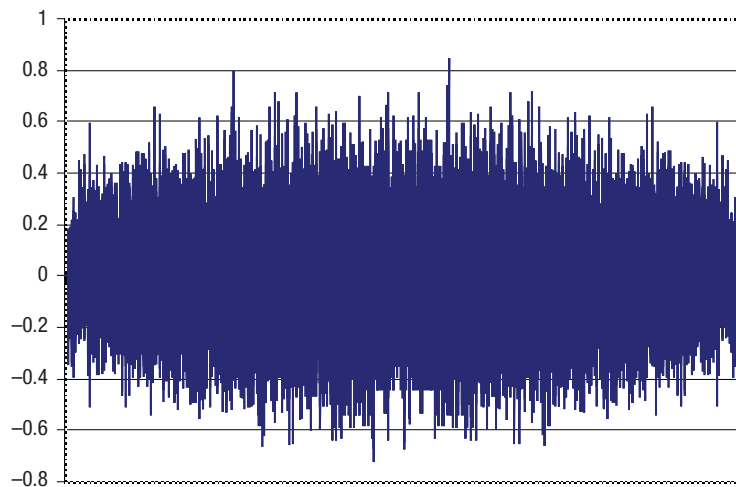
Figure 9. ADCDS-1603 Differential Nonlinearity, LSBs
