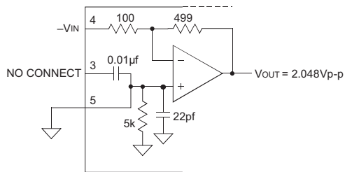
Figure 2e. Inverting Mode
